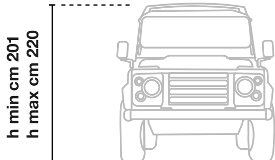
Changing room for 4x4 High-Wagon
